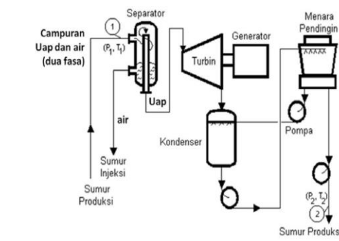
Figure 1. Flow Geothermal Power Plant Diagram
