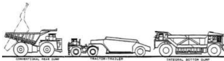
Figure 5. Truck Model
