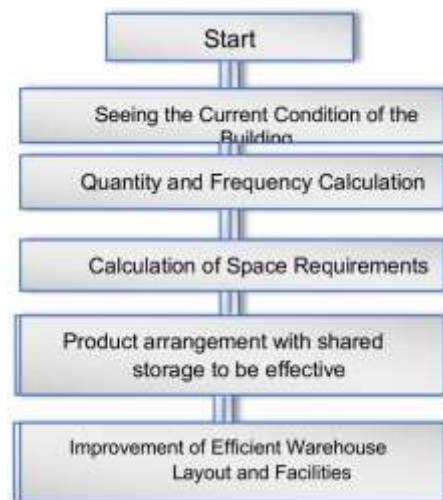
Figure 4. Framework Research
